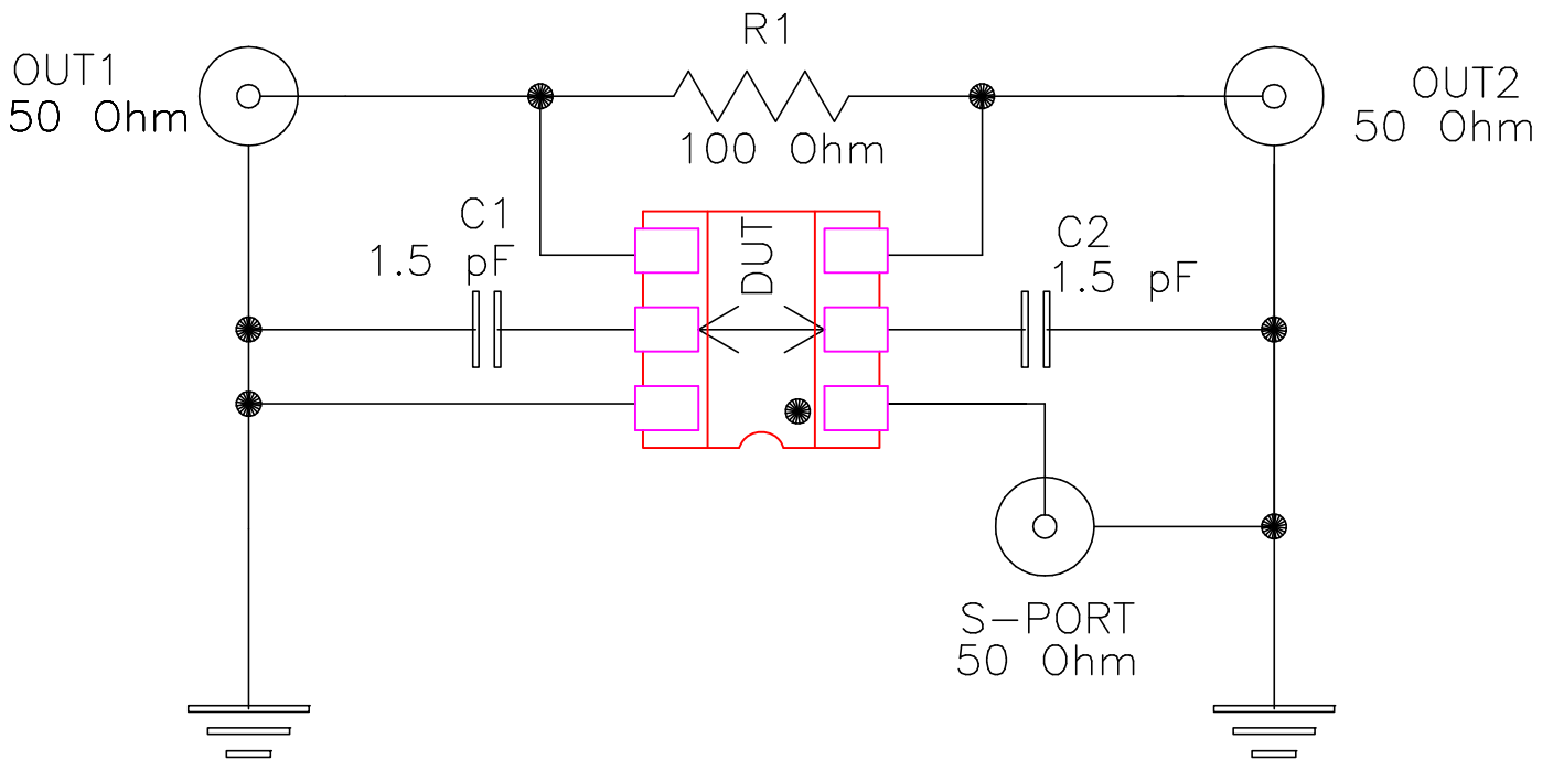
Schematic Diagram
