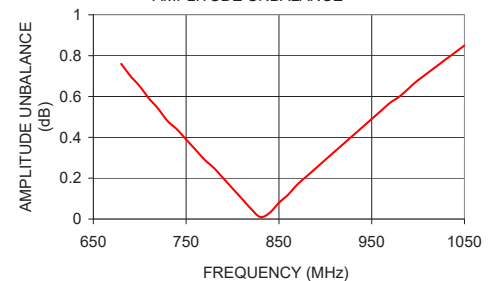
AMPLITUDE UNBALANCE
