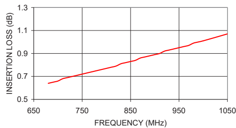
INSERTION LOSS
