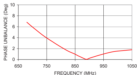
PHASE UNBALANCE
