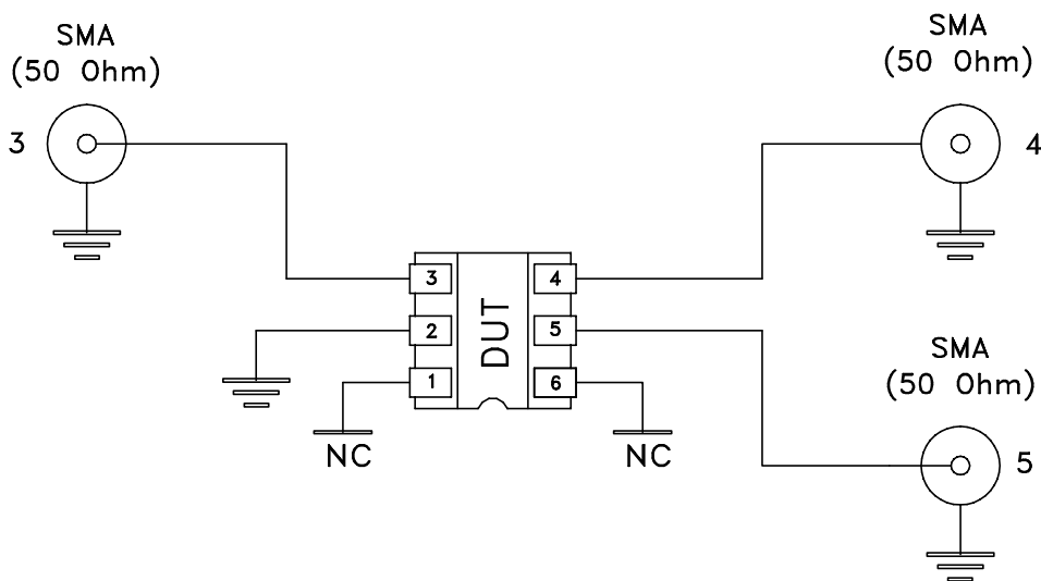
Schematic Diagram
