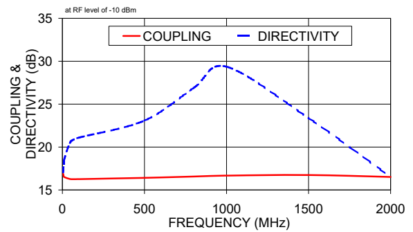
TCD-16-23-75X+ COUPLING & DIRECTIVITY
