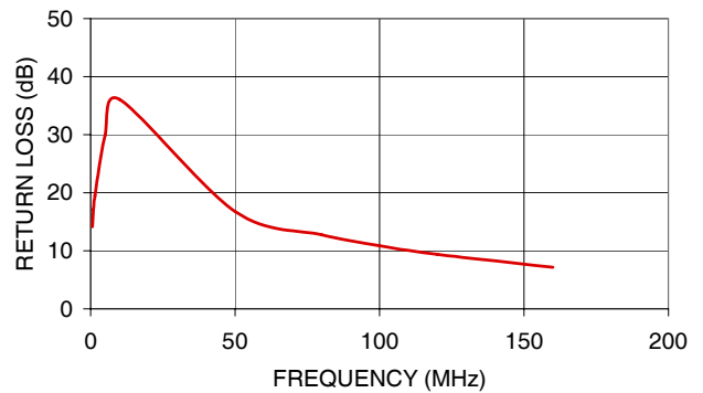
TC16-161T+ INPUT RETURN LOSS
