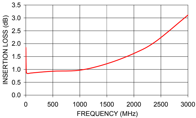
TC1-33-75G2A+ INSERTION LOSS
