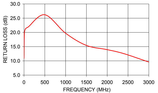
TC1-33-75G2A+ INPUT RETURN LOSS
