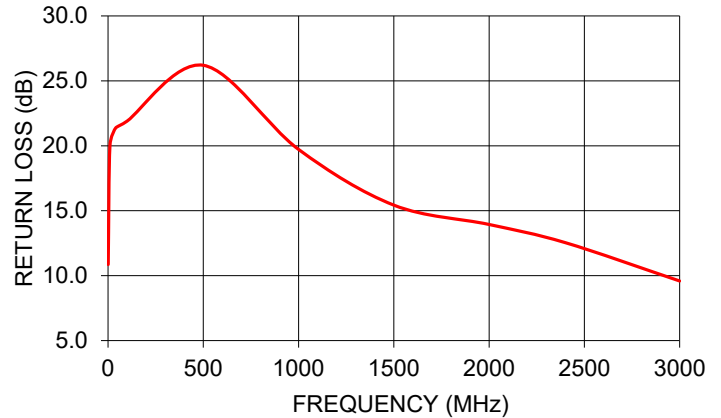
TC1-33-75-7+ INPUT RETURN LOSS
