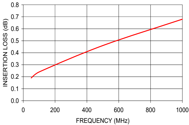
TC1-1-13M-22+ INSERTION LOSS
