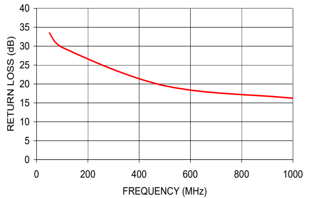
TC1-1-13M-22+ INPUT RETURN LOSS
