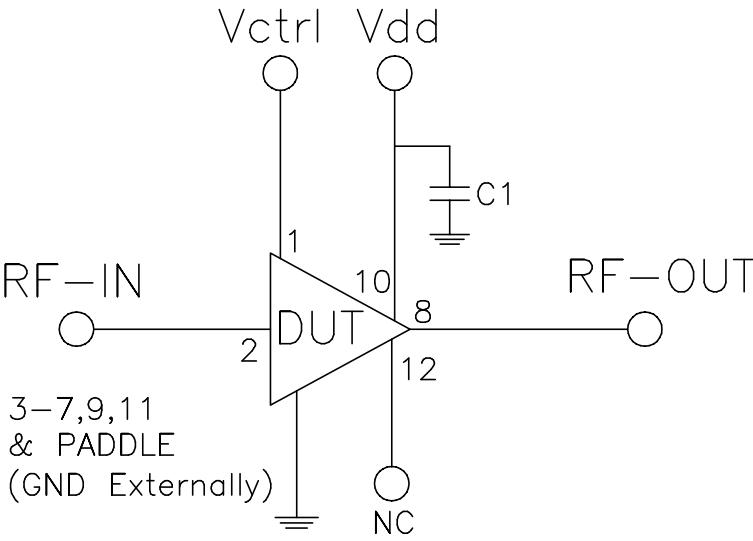
SCHEMATIC DIAGRAM
