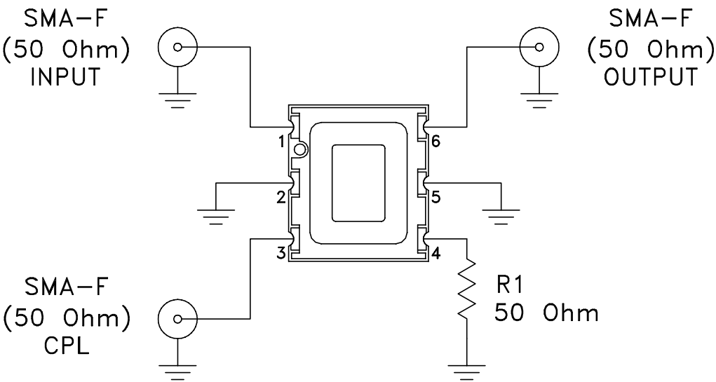
Schematic diagram
