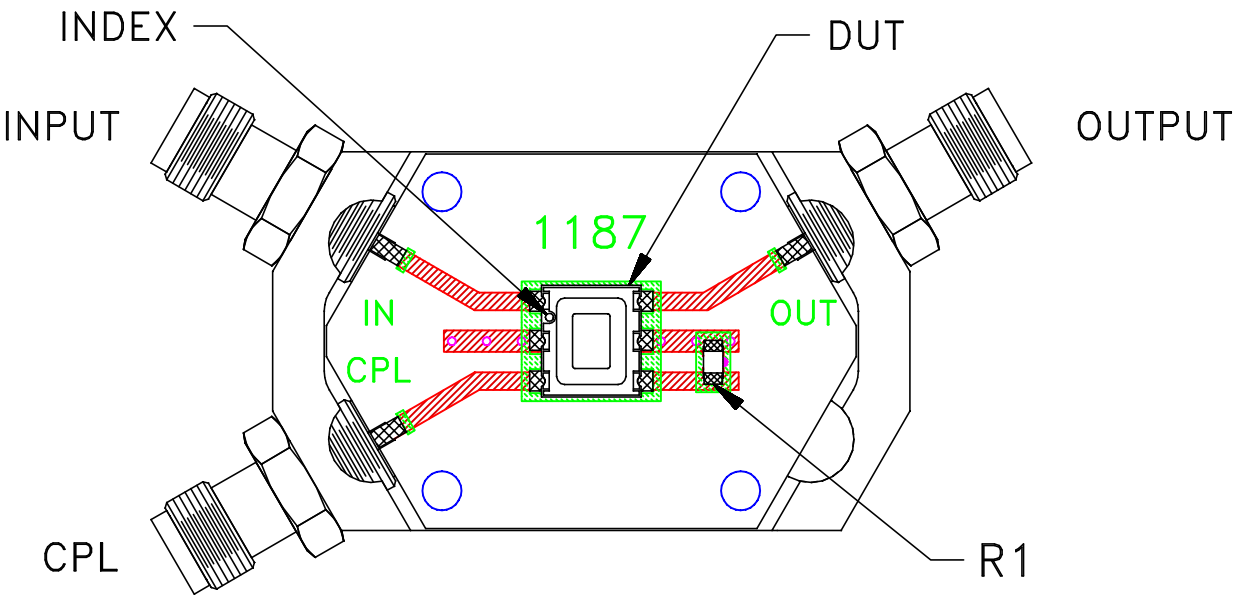
Schematic diagram
