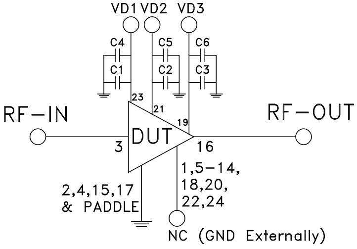
SCHEMATIC DIAGRAM
