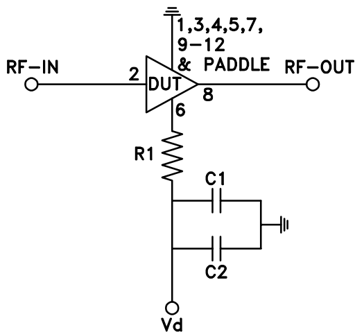
SCHEMATIC DIAGRAM
