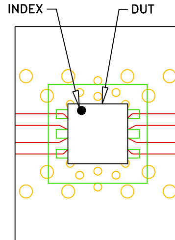
DETAIL "A" (SCALE 6:1)
