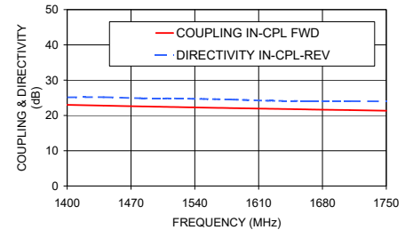
SYBD-22-172HP+ COUPLING & DIRECTIVITY
