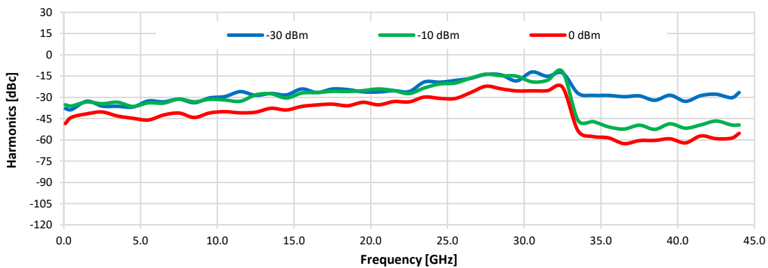
Sub-Harmonics (F1.5) vs. Output Frequency
