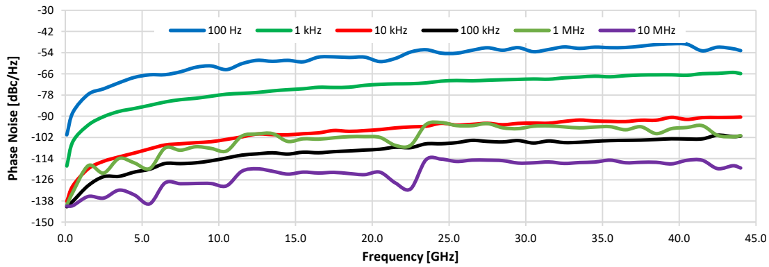
Phase Noise vs. Output Freq. at Frequency Offsets
