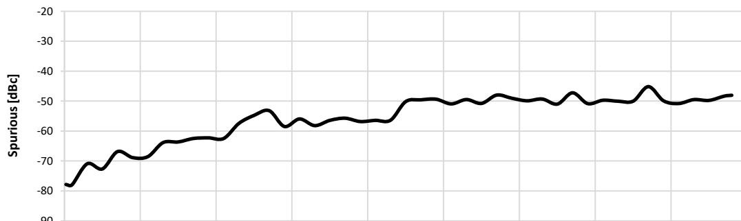
Spurious vs. Output Frequency @ -5 dBm
