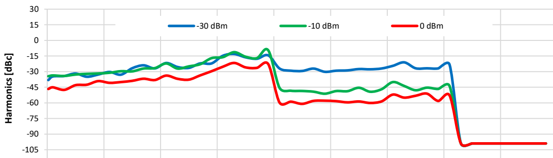
Sub-Harmonics (F2.5) vs. Output Frequency
