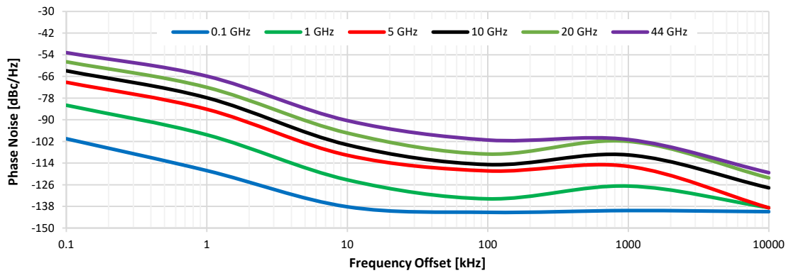
Phase Noise vs. Offset Freq. at Frequency Output
