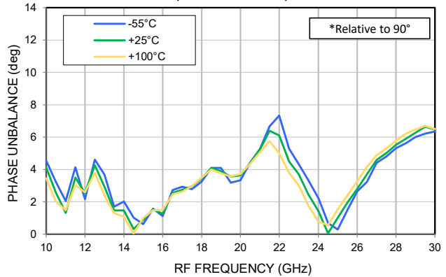
PHASE UNBALANCE* vs. TEMPERATURE IF = 200 MHz, LO = +18 dBm, RF = LO - IF
