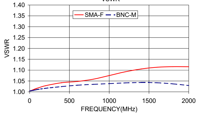
SF-BM50 VSWR
