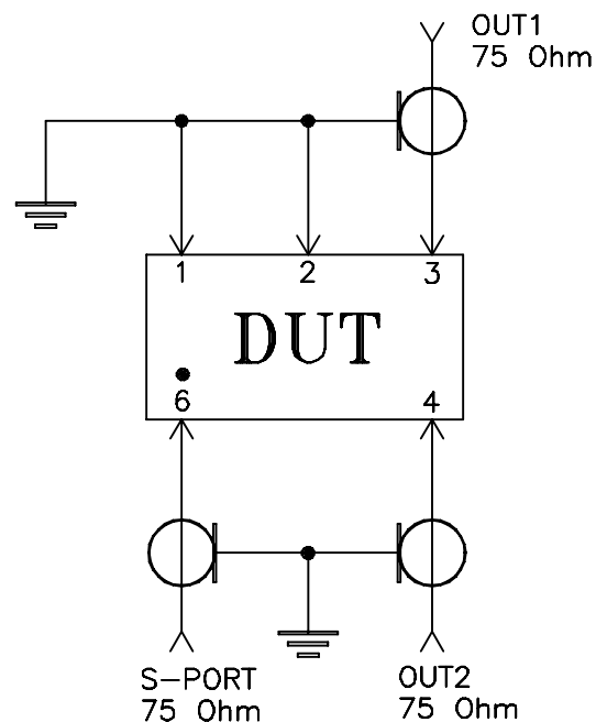
Schematic Diagram
