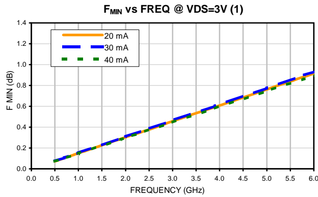
(1) F MIN is minimum Noise Figure
