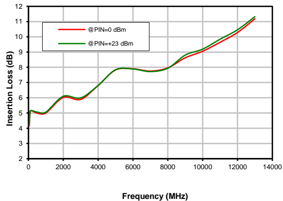
Insertion Loss
