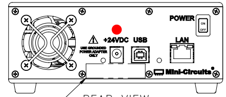
REAR VIEW
