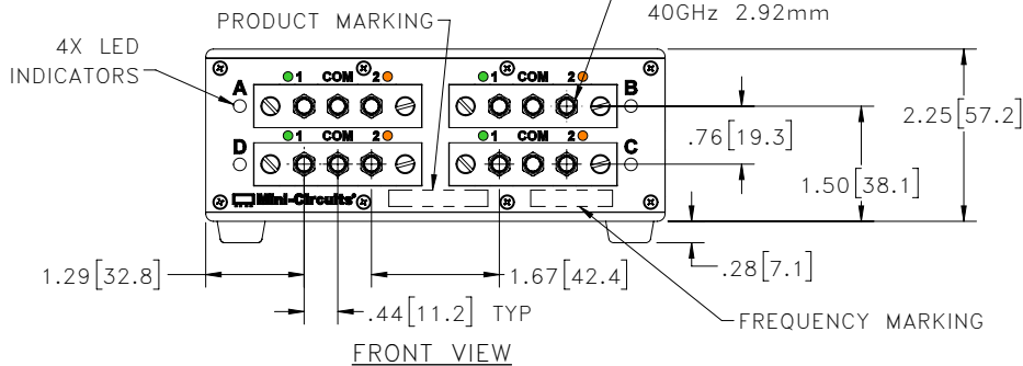
FRONT VIEW
