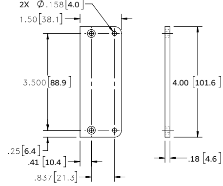
REAR VIEW BRACKET OPTION ONE SET OF 2 EACH
