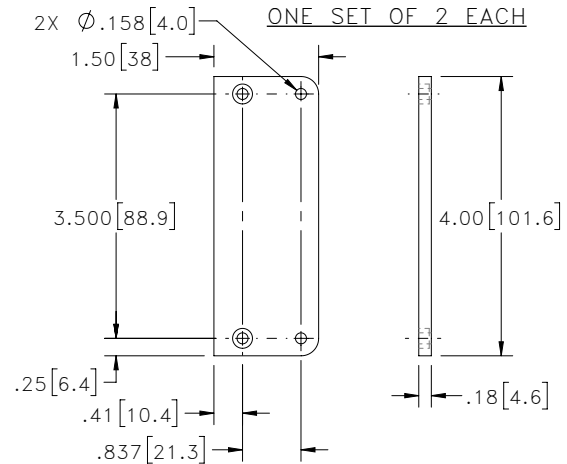
S/N LABEL BRACKET OPTION ONE SET OF 2 EACH
