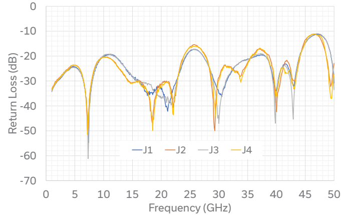
Return Loss
