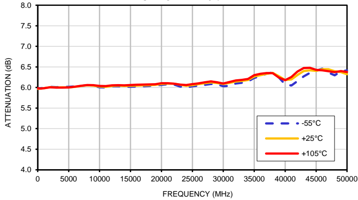
ATTENUATION vs. TEMPERATURE INPUT POWER = 0 dBm
