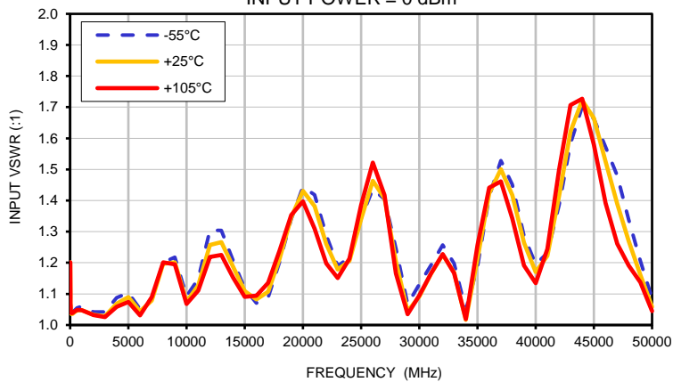
INPUT VSWR vs. TEMPERATURE
