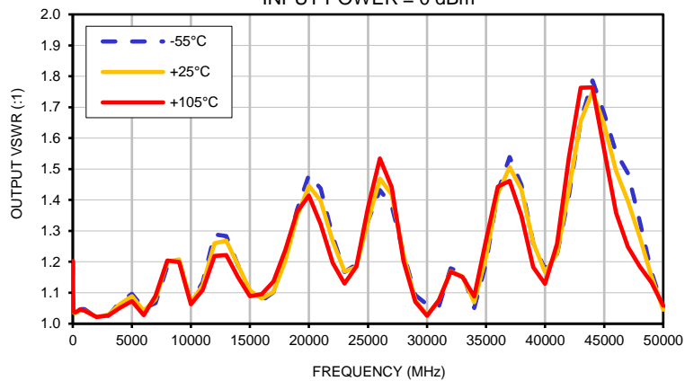
OUTPUT VSWR vs. TEMPERATURE
