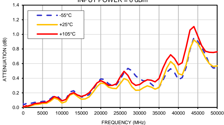
ATTENUATION vs. TEMPERATURE
