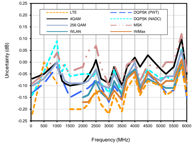
UNCERTAINTY OF POWER MEASUREMENT MODULATED SIGNAL @ 25°C
