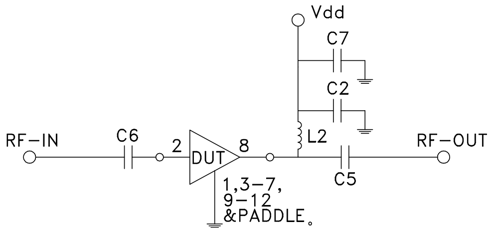
Schematic Diagram
