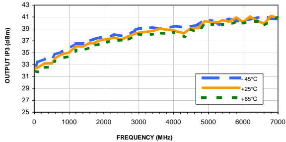
OUTPUT IP3 vs. FREQUENCY & TEMPERATURE
