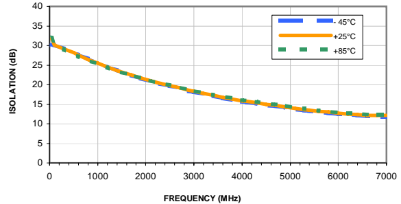
ISOLATION vs. FREQUENCY & TEMPERATURE Vd = 3V, Rbias=1K Ohms
