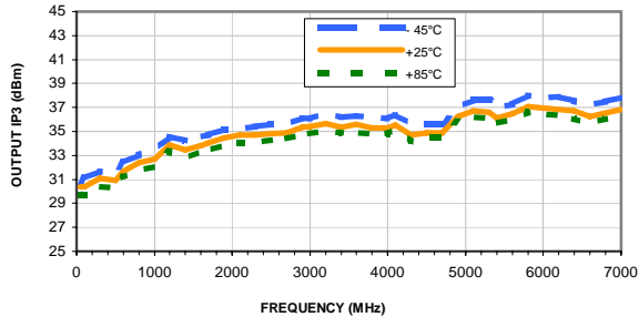
OUTPUT IP3 vs. FREQUENCY & TEMPERATURE Vd = 3V, Rbias=1K Ohms
