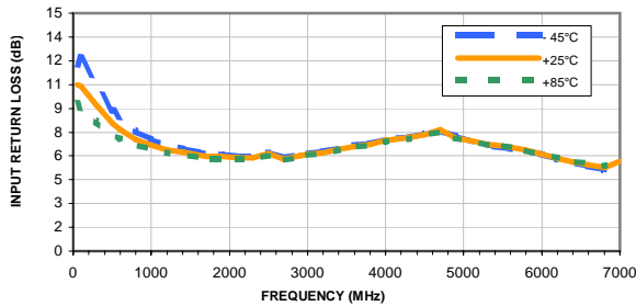
INPUT RETURN LOSS vs. FREQUENCY & TEMPERATURE Vd = 3V, Rbias=1K Ohms
