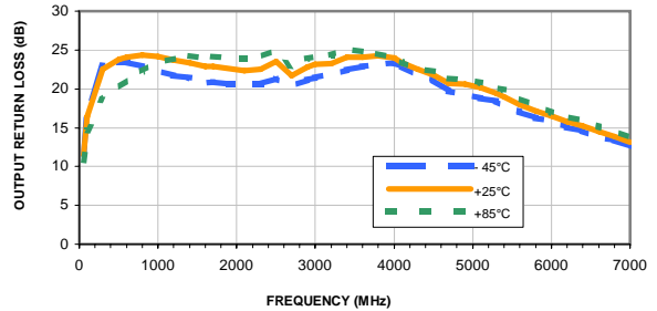
OUTPUT RETURN LOSS vs. FREQUENCY & TEMPERATURE Vd = 3V, Rbias=1K Ohms
