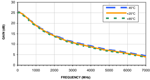
GAIN vs. FREQUENCY & TEMPERATURE Vd = 3V, Rbias=1K Ohms
