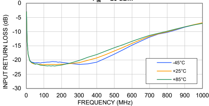
INPUT RETURN LOSS vs. TEMPERATURE P_{IN} = -25\text{ dBm}
