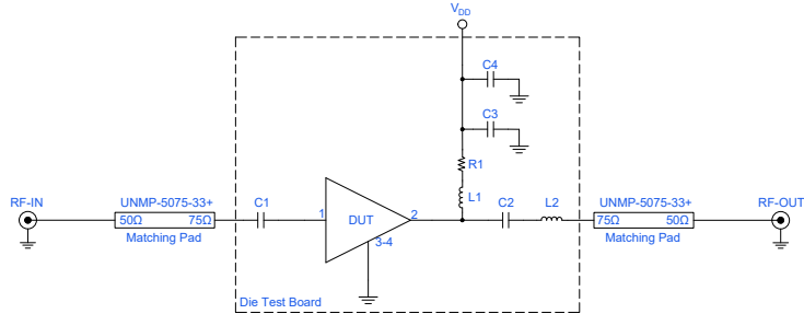
Figure 3. PGA-32-75-D+ Characterization Circuit
