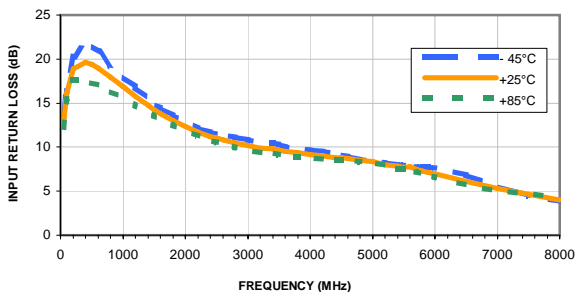
INPUT RETURN LOSS vs. FREQUENCY & TEMPERATURE INPUT POWER = -25dBm, Vd = 3.3V
