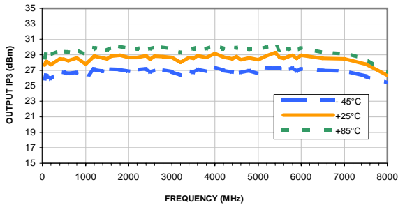
OUTPUT IP3 vs. FREQUENCY & TEMPERATURE OUTPUT POWER = 0 dBm/tone, Vd = 3.3V
