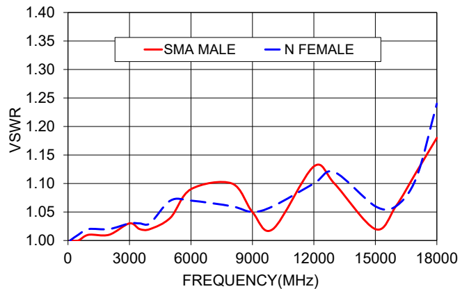
NF-SM50+ VSWR
