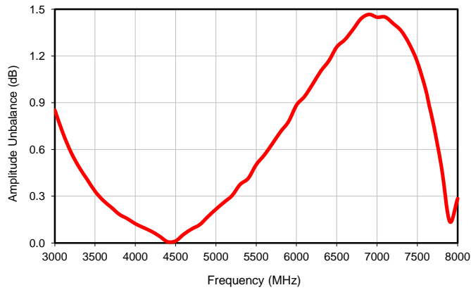
Amplitude Unbalance
