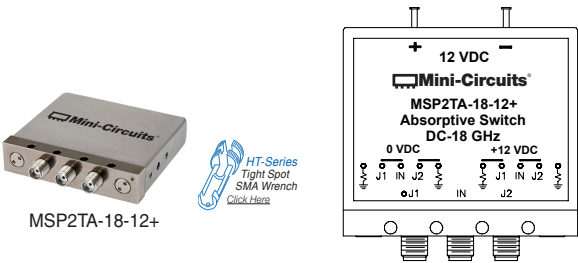
Marking Drawing
