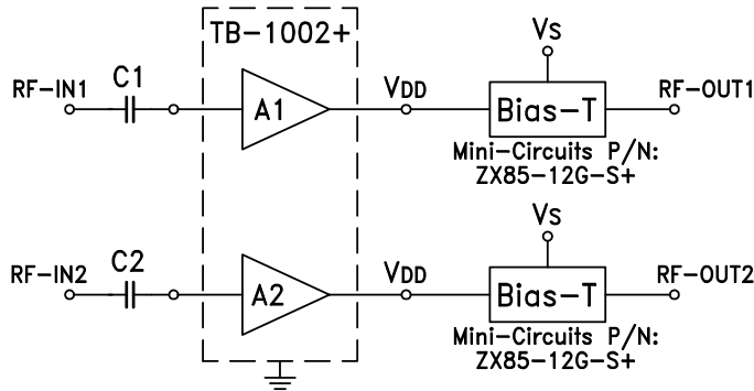
Fig 1. Block Diagram of Test Circuit used for characterization. (DUT tested in Mini-Circuits Test board TB-1002+). Gain, Return loss, Output Power at 1dB compression (P1 dB), output IP3 (OIP3) and noise figure measured using Agilent’s N5242A PNA-X micro-wave network analyzer.
