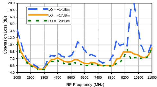
Conversion Loss vs. LO @ RF=5400MHz
