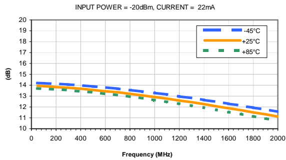
GAIN vs. TEMPERATURE
