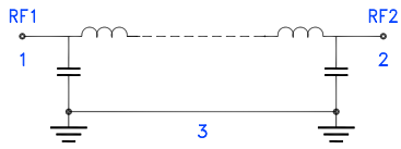
Figure 1. LFHK-4800+ Functional Diagram
