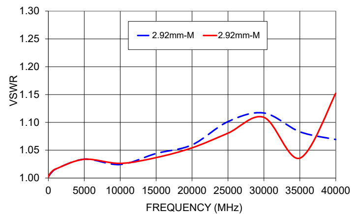
KMR-KM50+ VSWR
