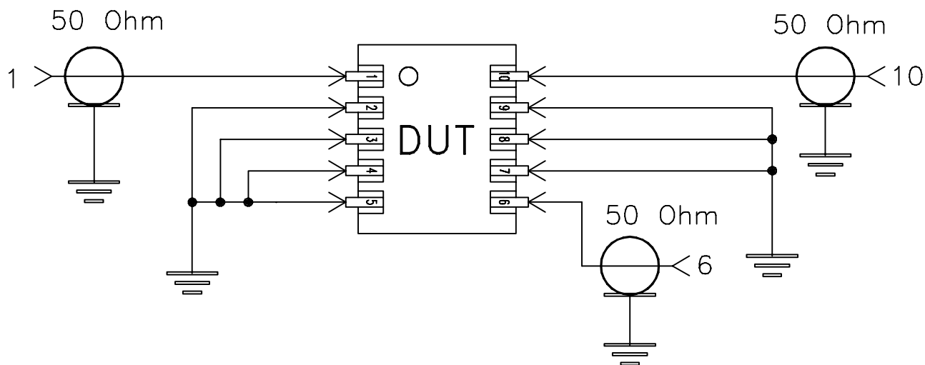
Schematic Diagram
