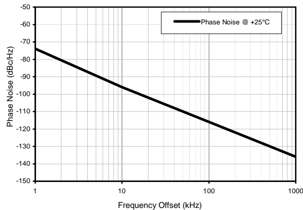
Phase Noise
