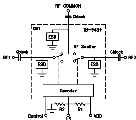
Figure 1. Block Diagram of test Circuit used for characterization (DUT, R1&R2 soldered on Mini-Circuit's TB-948+) R1=2.21kΩ R2=3.32kΩ (can be omitted if V DD =2.3 to 3.3V)
