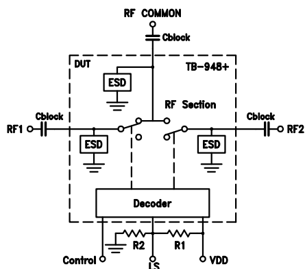
Figure 1. Block Diagram of test Circuit used for characterization (DUT, R1&R2 soldered on Mini-Circuit's TB-948+) R1=2.21kΩ R2=3.32kΩ (can be omitted if V DD =2.3 to 3.3V)
