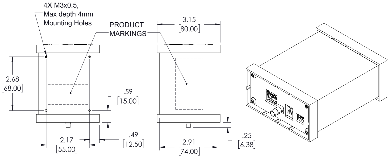
BOTTOM VIEW
