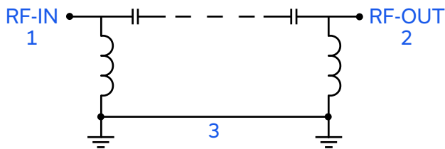
Figure 1. HFCU-1582+ Functional Diagram
