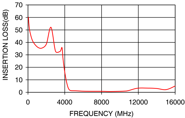
HFCN-4400+ INSERTION LOSS
