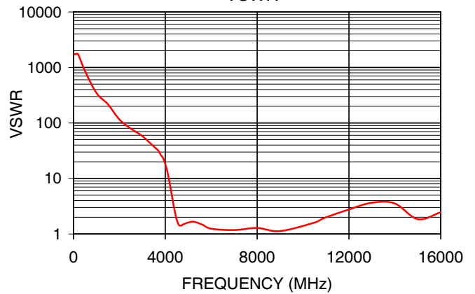
HFCN-4400+ VSWR
