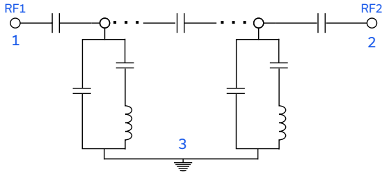
Figure 1. HFCN-3052+ Functional Diagram
