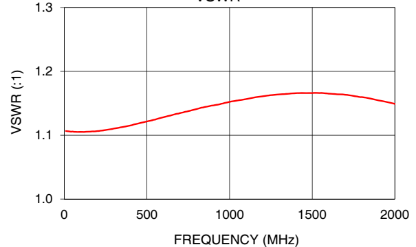
HAT-9A+ VSWR
