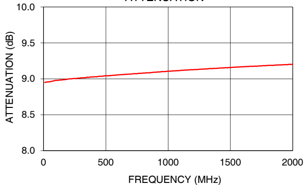
HAT-9A+ ATTENUATION
