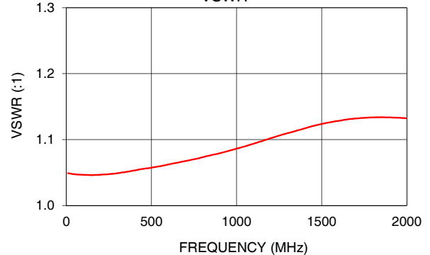
HAT-6A+ VSWR
