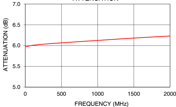
HAT-6A+ ATTENUATION
