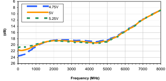
OUTPUT RETURN LOSS vs. DEVICE VOLTAGE
